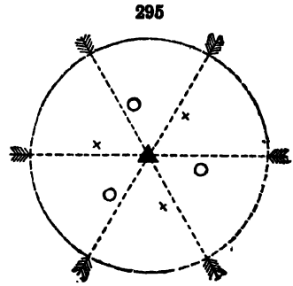
Symmetry of Tri-Rhombohedral Class
